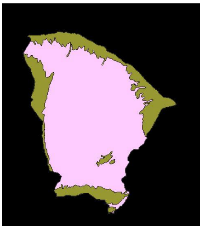
Figure 1. The State of Ceará and its geological configuration. Crystalline basement is located in central area, while sediments (State edges) are located in all other areas.
