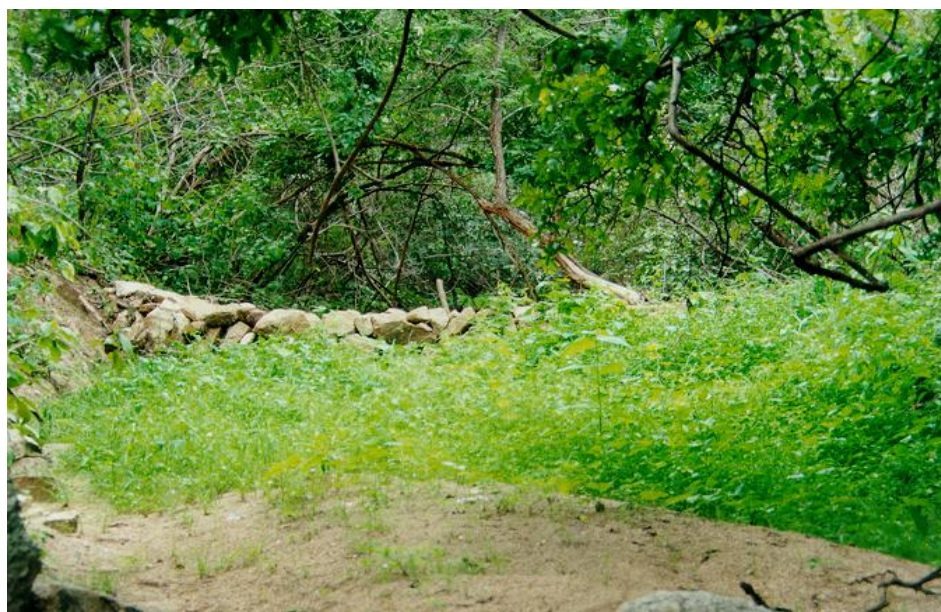
Figure 6 – Effect of sediment retention and reappearance of arborous and herbaceous vegetation after winter period.
