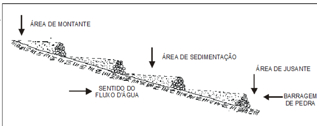
Figure 3 – Stone dam sequence.
