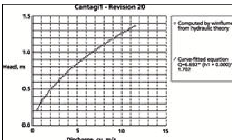
Figure 2.110 – Theoretical key curve of flume 1 (Salgadinho stream)
