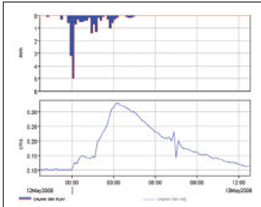
Figure 2.112 – Hydrogram seen in 05/12/2008 event in Salgadinho stream
