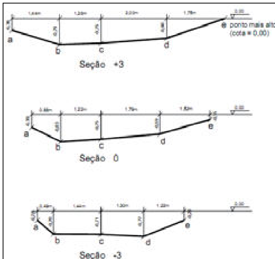
Figure 2.01 – Cross sections of flume 01
