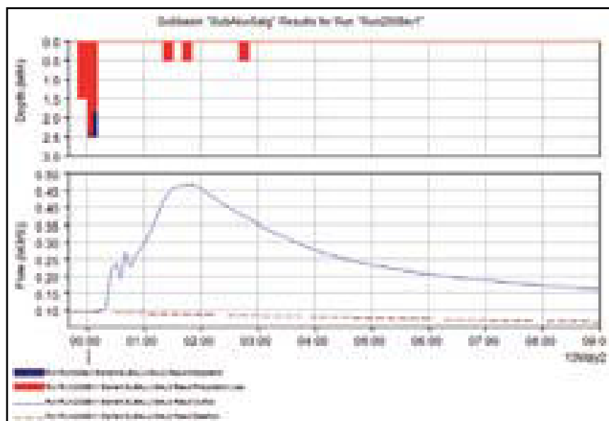
Figure 2.126 – Simulation of a flood event in 2008 (Salgadinho stream)
